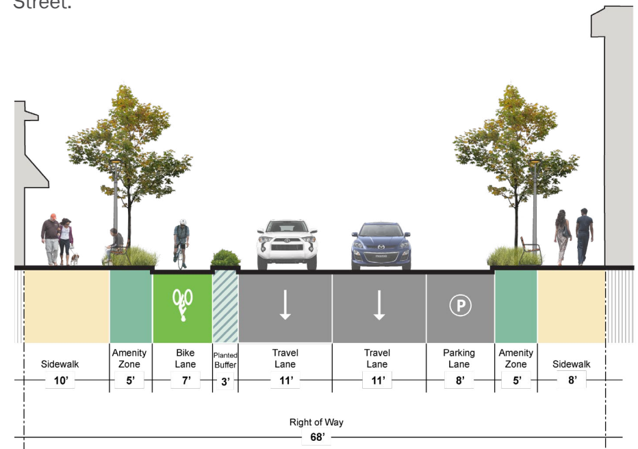
Section A illustrates protected bike lane and wider sidewalks along Main Street.
