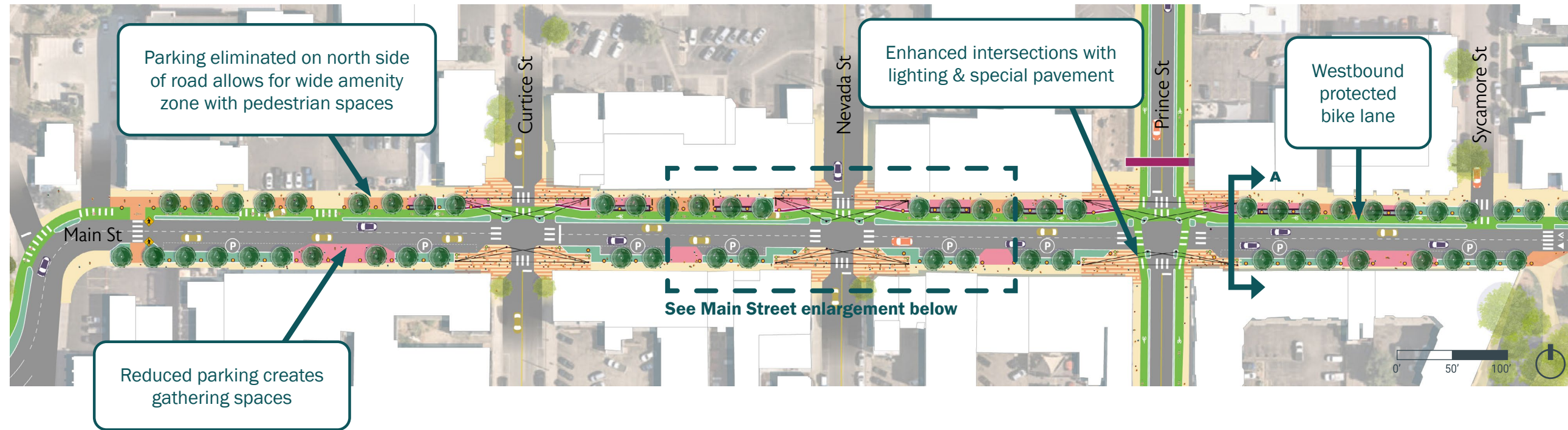
Section A illustrates protected bike lane and wider sidewalks along Main Street.
