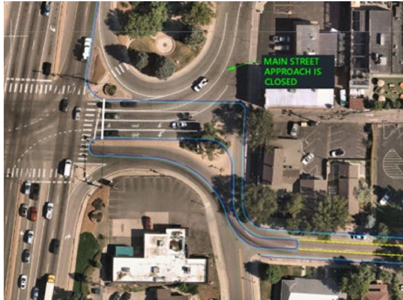
Figure 21: Alamo Avenue & Santa Fe Drive/Bowles Avenue – Option A
