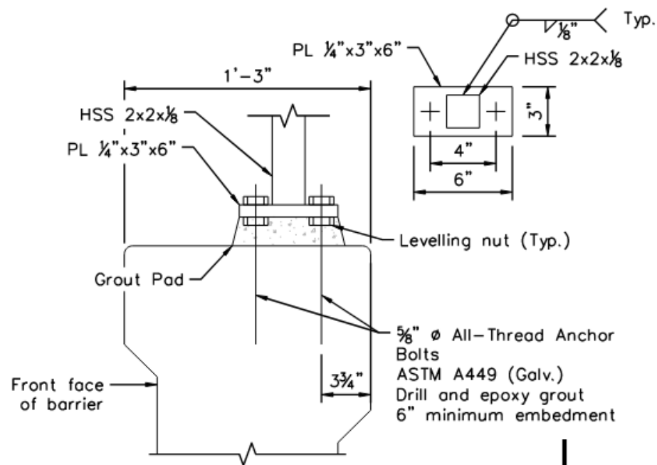
4 11 MONUMENT BASE PLATE SECTION
