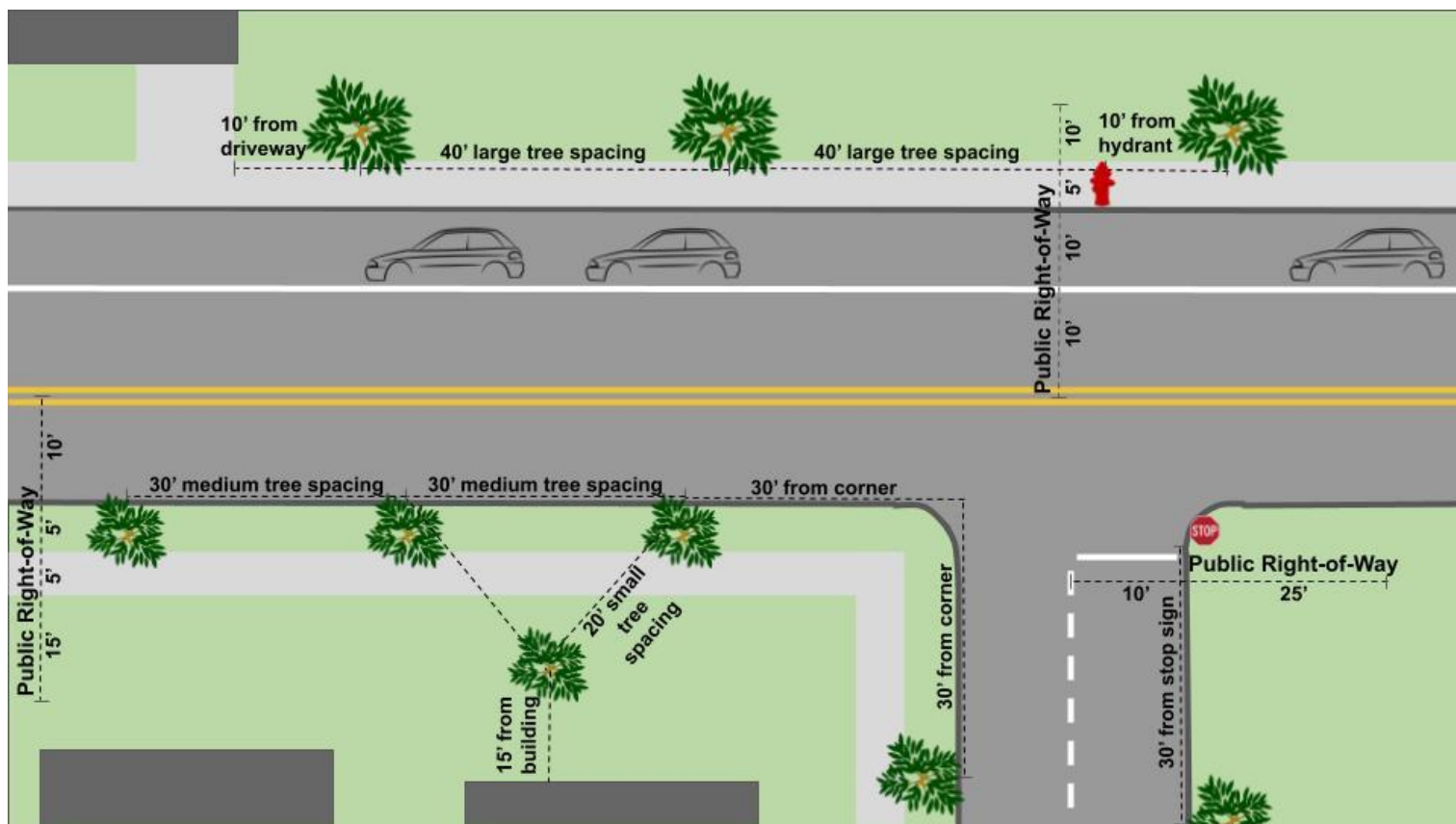
Figure 1. Street layout depicting the typical ROW size and several minimum spacing requirement examples (see Table 2 for full list).
